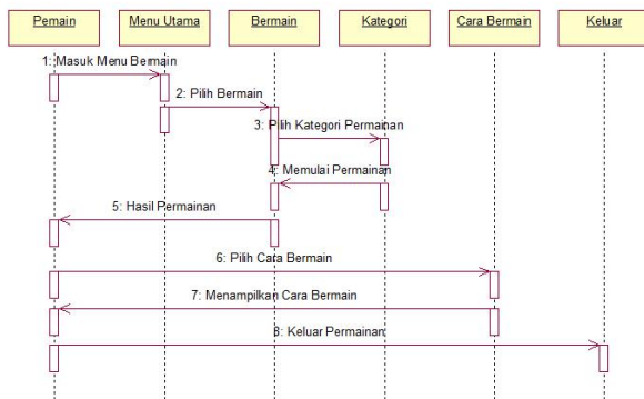
Gambar 4. Sequence Diagram Edugame Guess The Country
