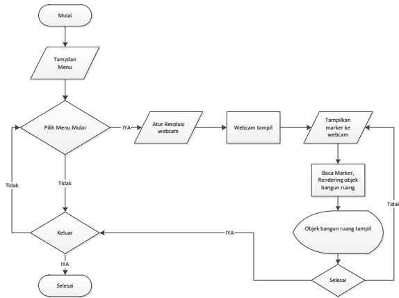
Gambar 4. Flowchart Program
