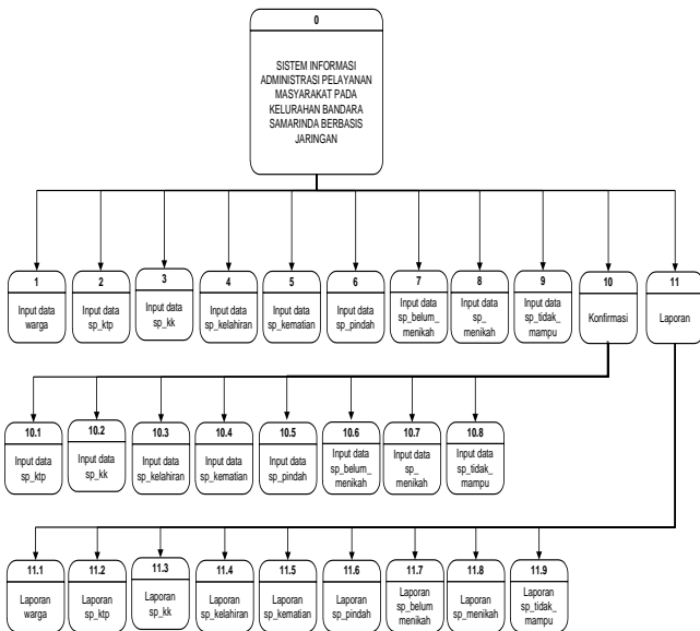
Gambar 2. Hierarchy Input Process Output (HIPO)
