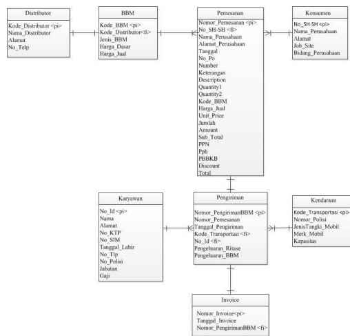
Gambar 8 Entity Relationship Diagram (ERD)
