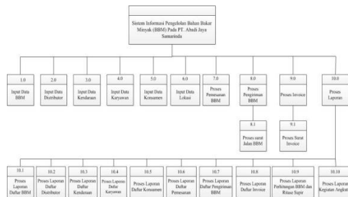
Gambar 7 Hierarchy Input Proses Output (HIPO)
