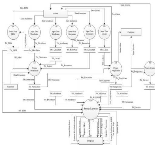
Gambar 4. Diagram Level 0 (DFD)
