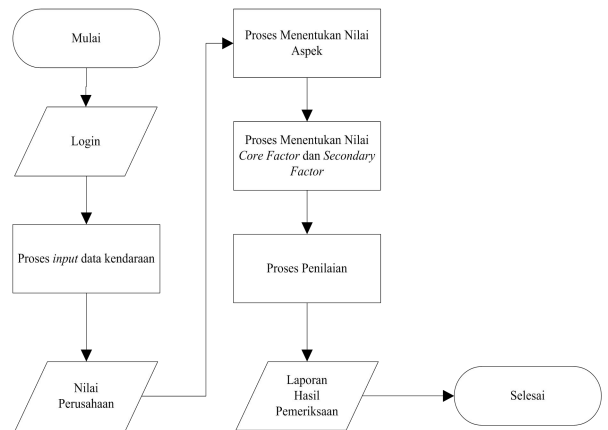
Gambar 6. Flowchart Program
