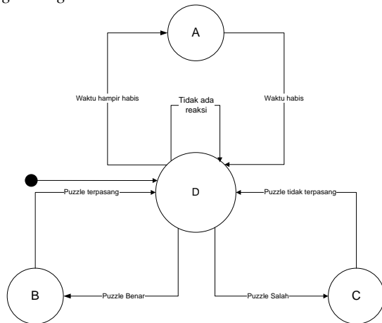
Gambar 4.1 Rancangan FSM ( Finite State Machine ).
